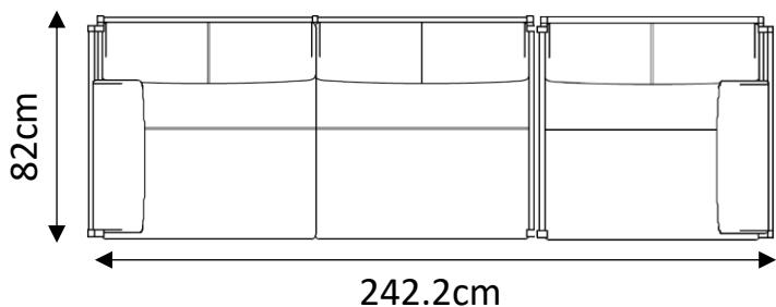
One Arm Sofa 160 (R) W159.6 .D82 .H73 .SH37
