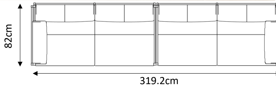
One Arm Sofa 160 (R) W159.6 .D82 .H73 .SH37
